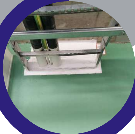
Fire Stopping/ Sealing Application
